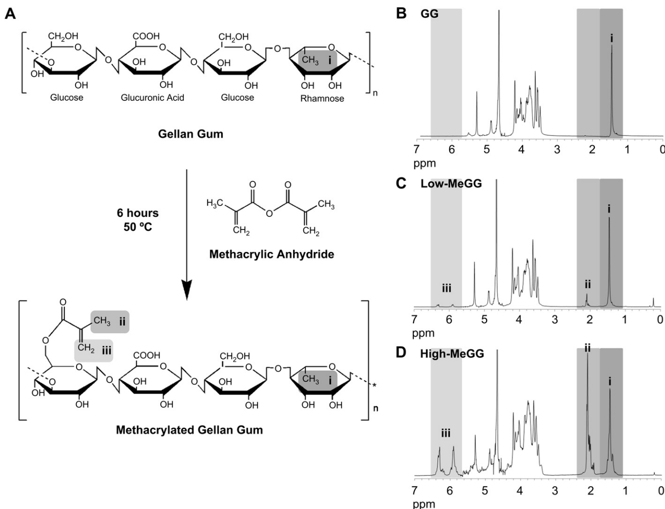
Fig. 1. (A) Schematic illustration of the synthesis of MeGG. ^1\text{H} NMR spectra ( T = 50\text{ }^{\circ}\text{C} ) of (B) GG, (C) Low-MeGG and (D) High-MeGG recorded in \text{D}_2\text{O} . Methyl group of the MA (ii) was located at \delta 2.09 ppm and vinyl groups of the MA (iii) were identified around \delta 5.5–7 ppm.
